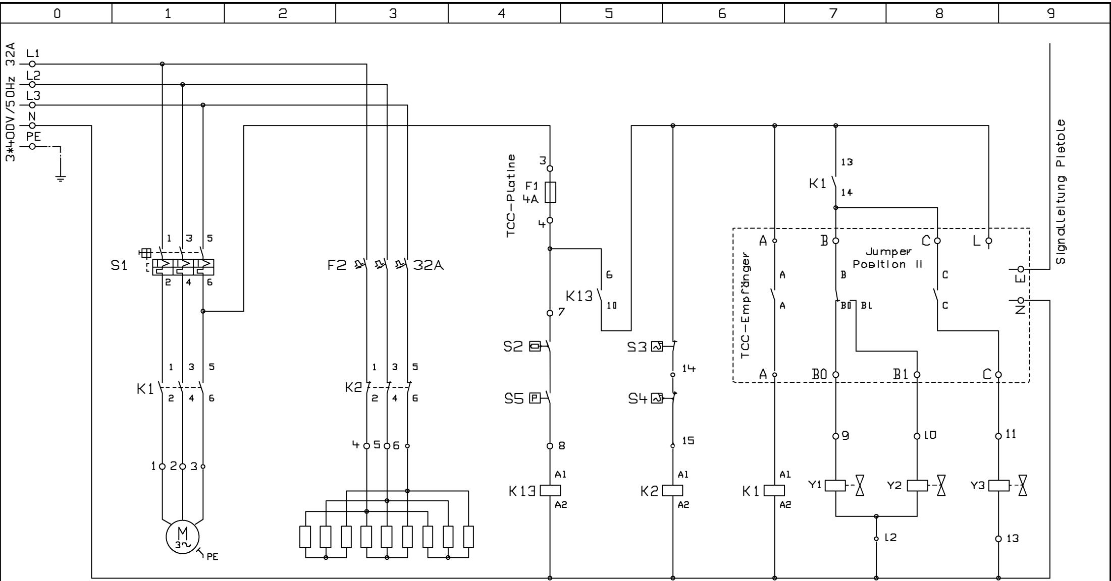
HD-Pumpe
